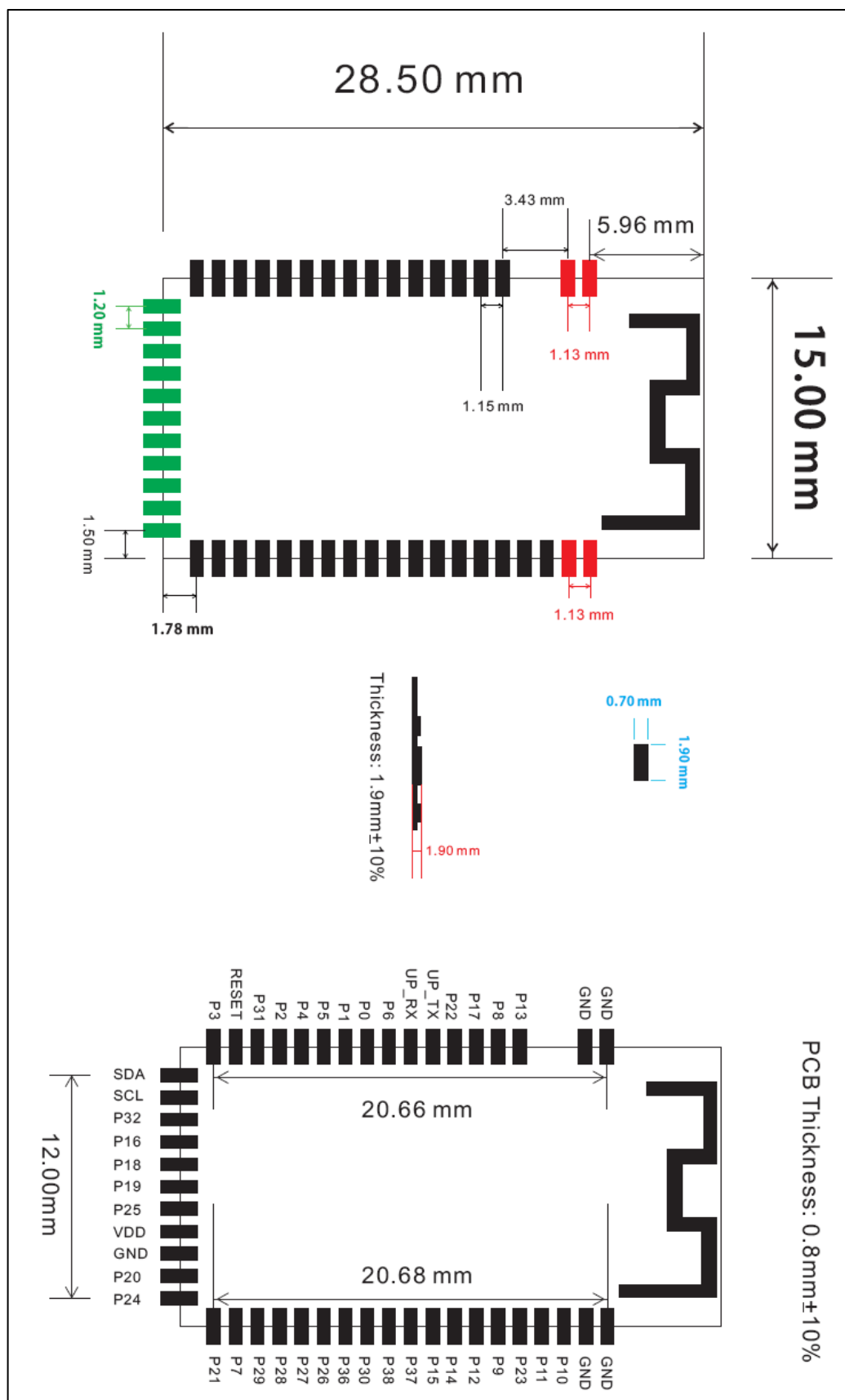
Figure 5: 47Pin-Bluetooth Module
