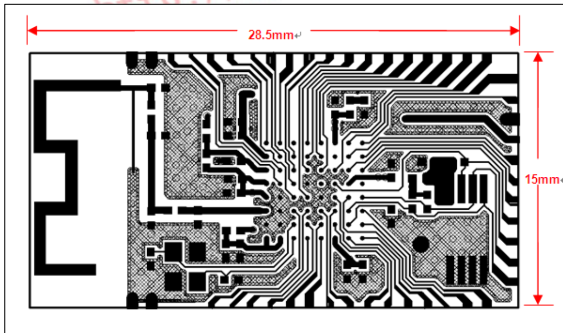
Figure 2: Module PCB Top View
