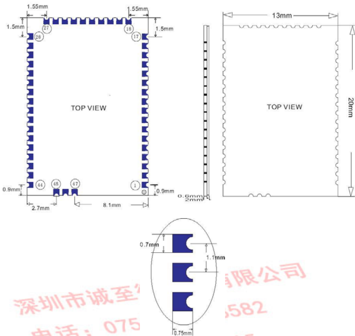
Figure 2: HZ-BC5 尺寸和脚位排列
