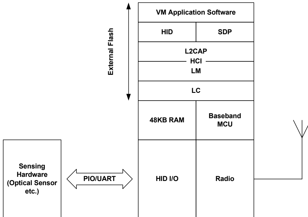
Figure 9.4: HID Stack
