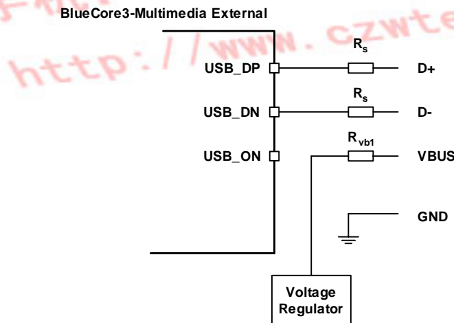
Figure 8.24: USB Connections for Bus-Powered Mode
