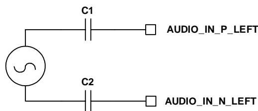
Figure 8.30: Differential Input (Left Channel Shown)
