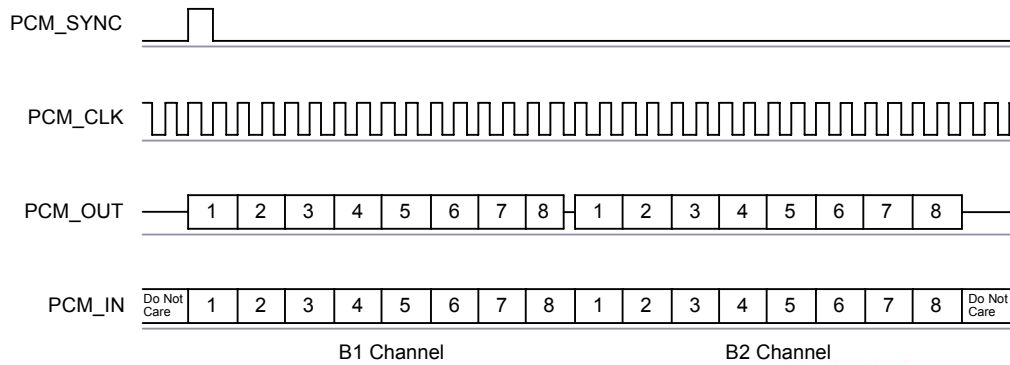
Figure 10.13: GCI Interface
