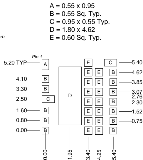
Solder Mask Pattern
