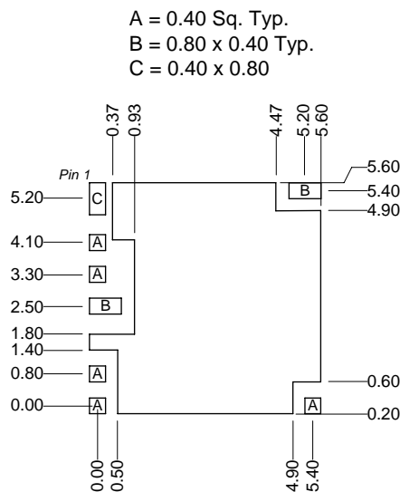
Metal Land Pattern
